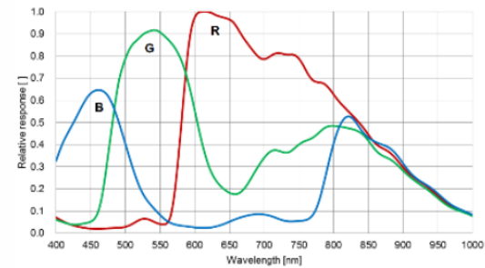
MV-CH089-10GM
