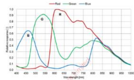
MV-CH089-10UC
