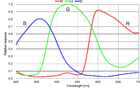
MV-CB120-10UC-B
